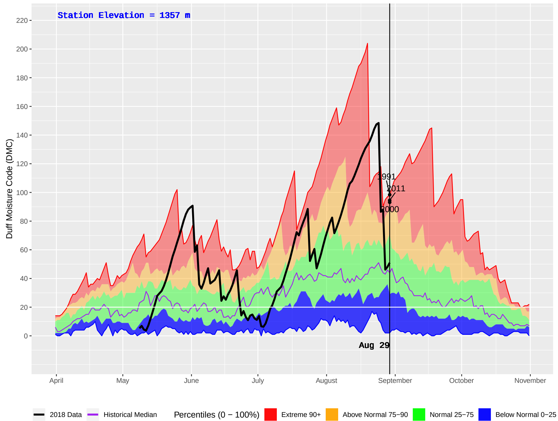
WHITE RIVER (790) : Historical (1989–2016) and Current (2018) Daily Duff Moisture Code (DMC)
